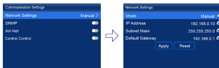
Figure 7-2 Network settings
