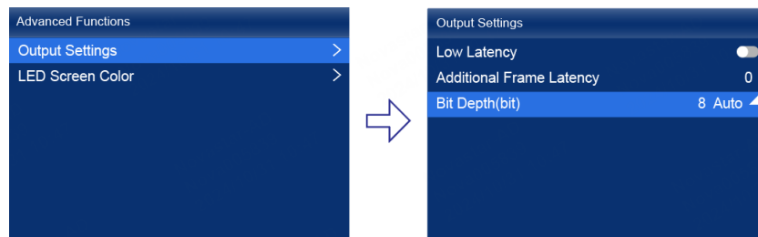
Figure 6-14 Bit depth
