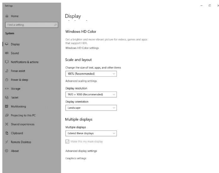
Figure 11-7 Multiple displays-2
