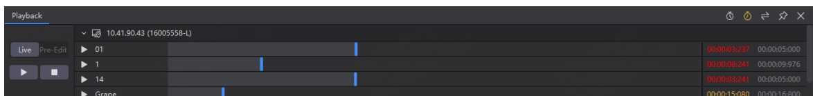
Figure 3-9 Playback control
