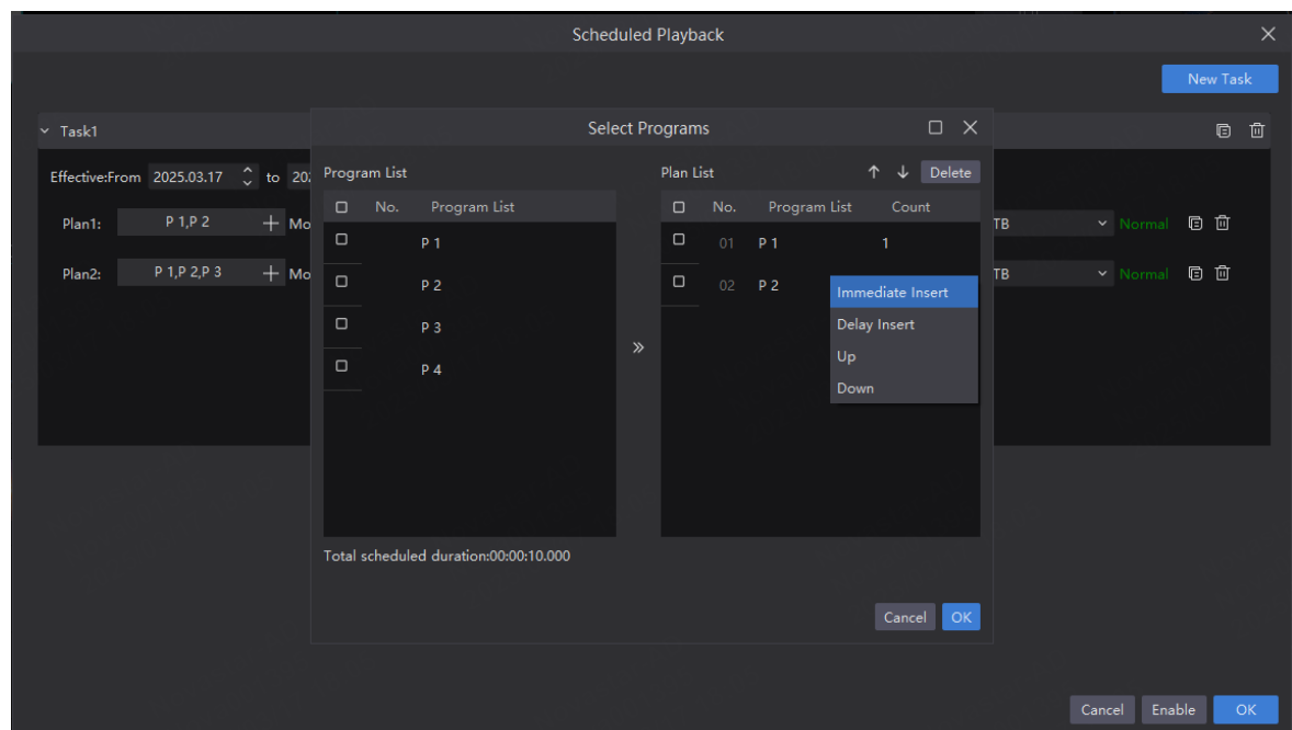
Figure 4-56 Insert programs
