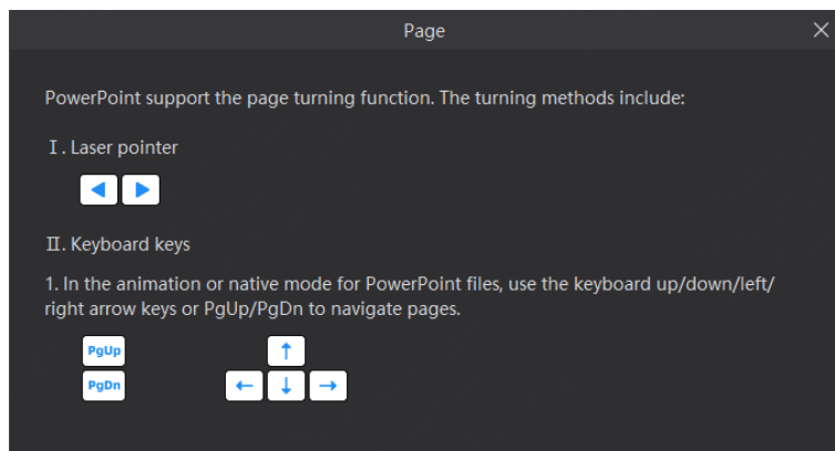
Figure 4-49 Page turning
