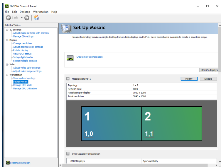
Figure 11-33 Mosaic completed
