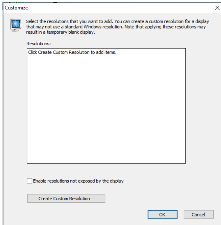
Figure 11-11 Custom resolution-1
