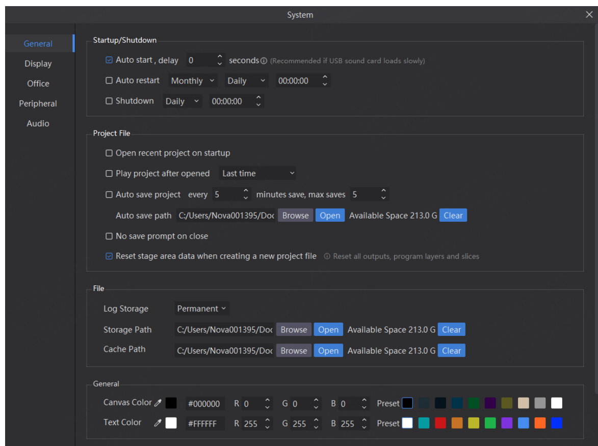
Figure 6-1 System settings
