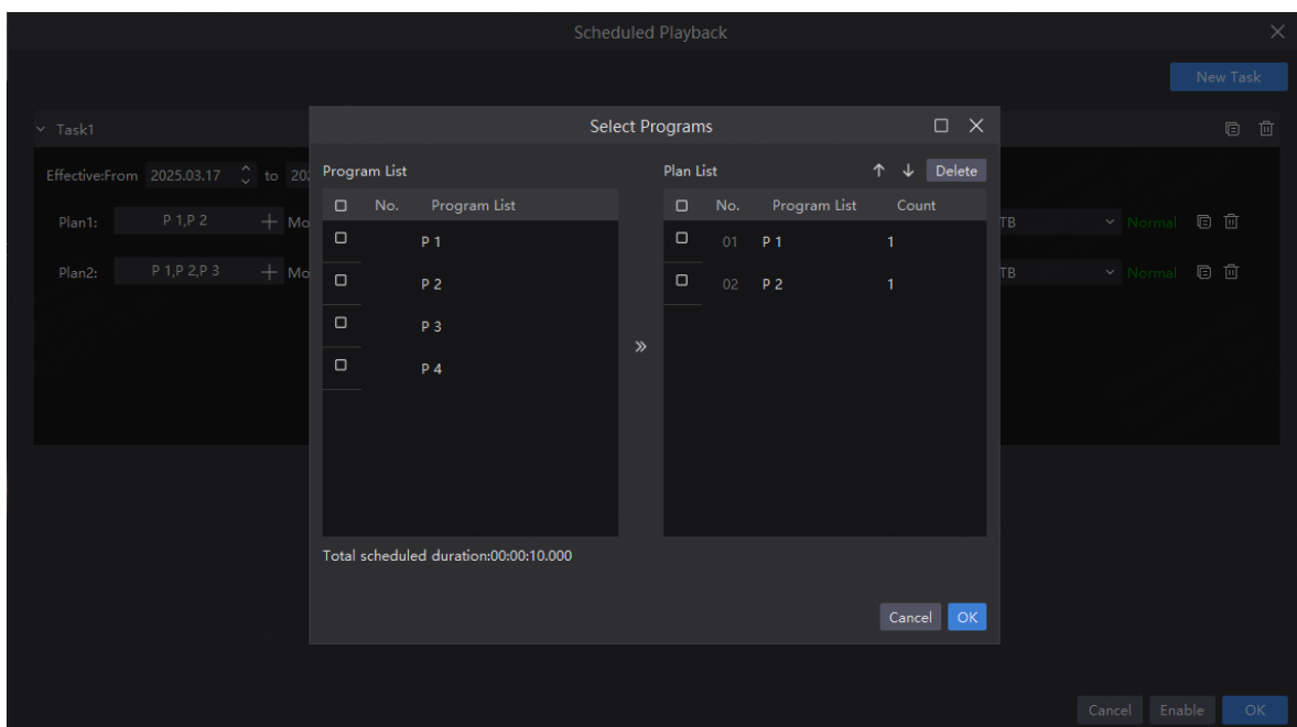
Figure 4-55 Select programs
