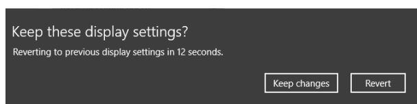
Figure 11-4 Confirmation
