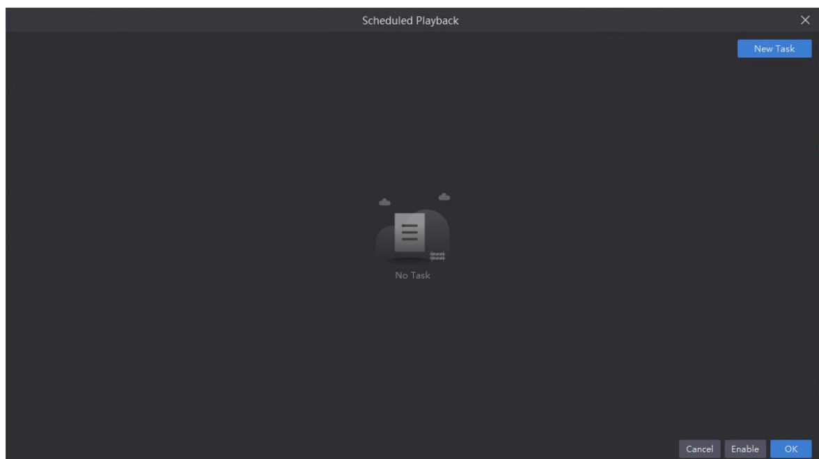
Figure 4-50 Scheduled playbacks
