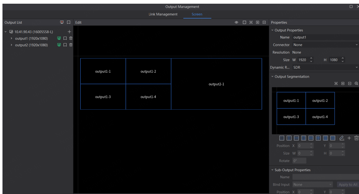
Figure 4-11 Screen management
