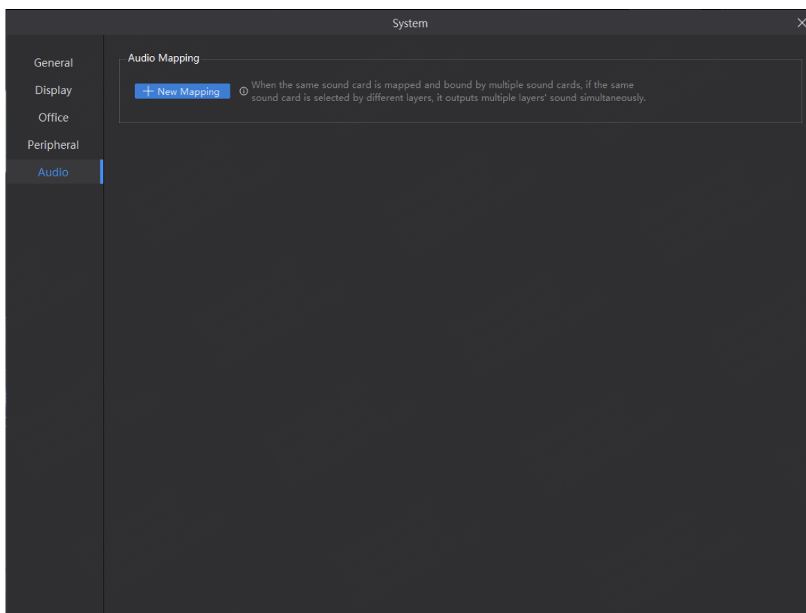
Figure 6-5 Audio settings
