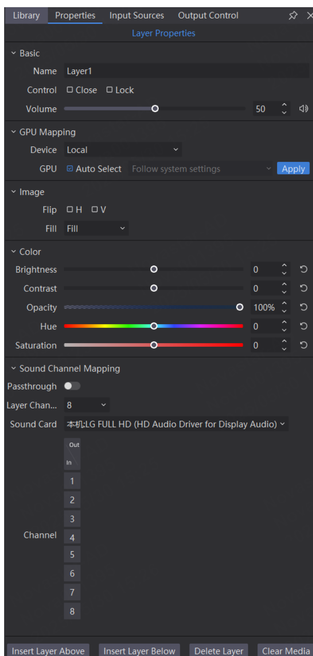
Figure 4-23 Layer properties
