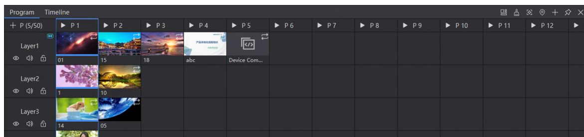
Figure 3-7 Program management
