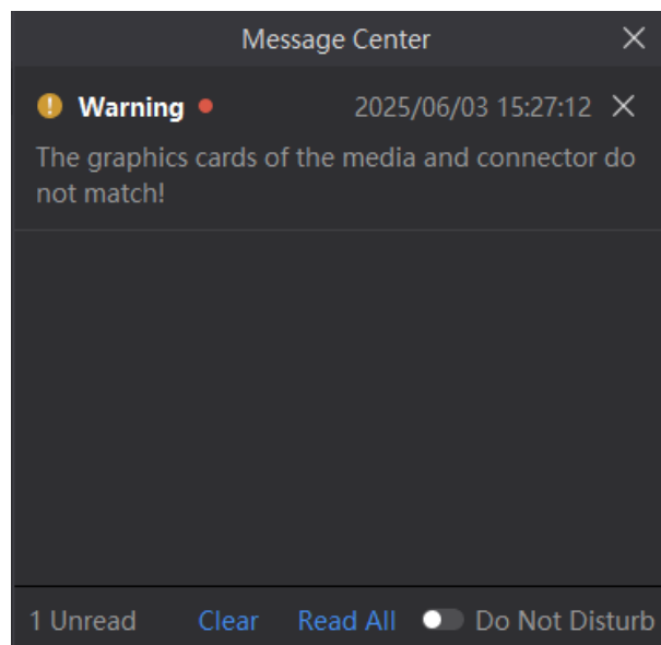
Figure 3-5 Message center
