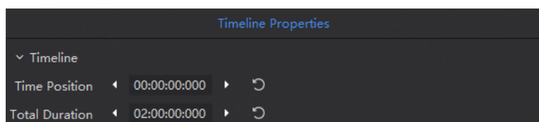
Figure 4-30 Timeline properties
