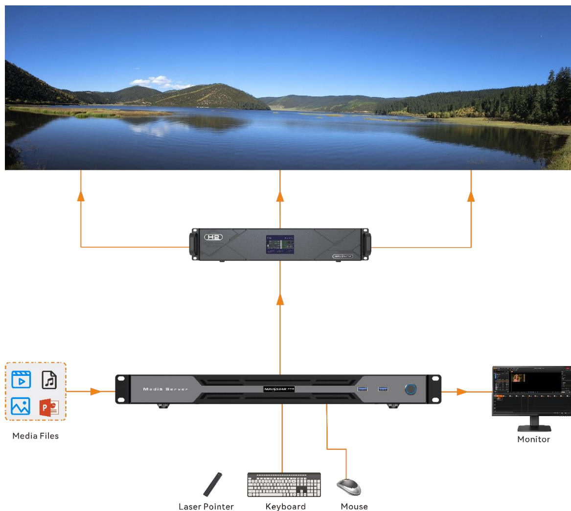
Figure 2-1 Application scenarios
