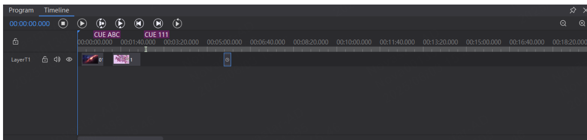
Figure 3-8 Timeline management
