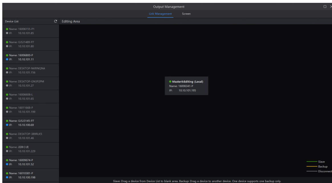
Figure 5-2 Link settings
