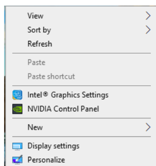
Figure 11-5 Display settings
