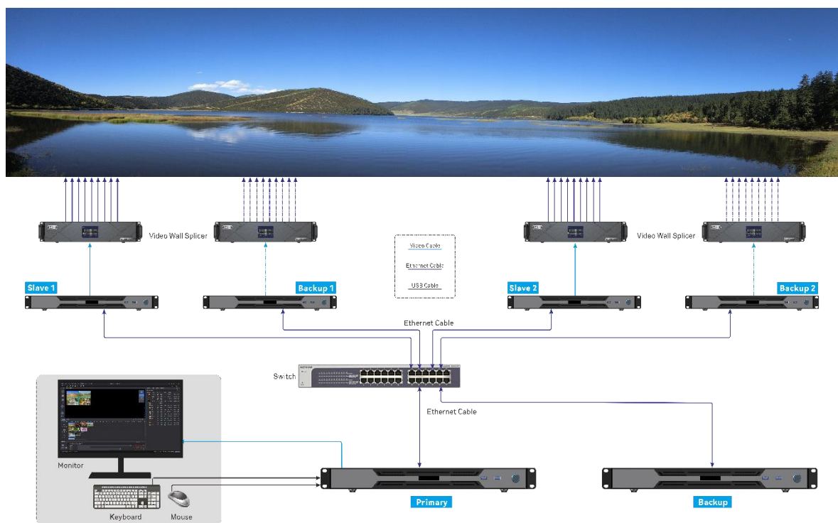
Figure 5-1 Application scenarios
