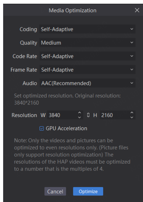
Figure 4-3 Media optimization
