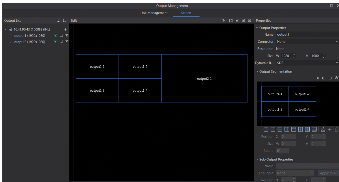
Figure 4-12 Output segmentation
