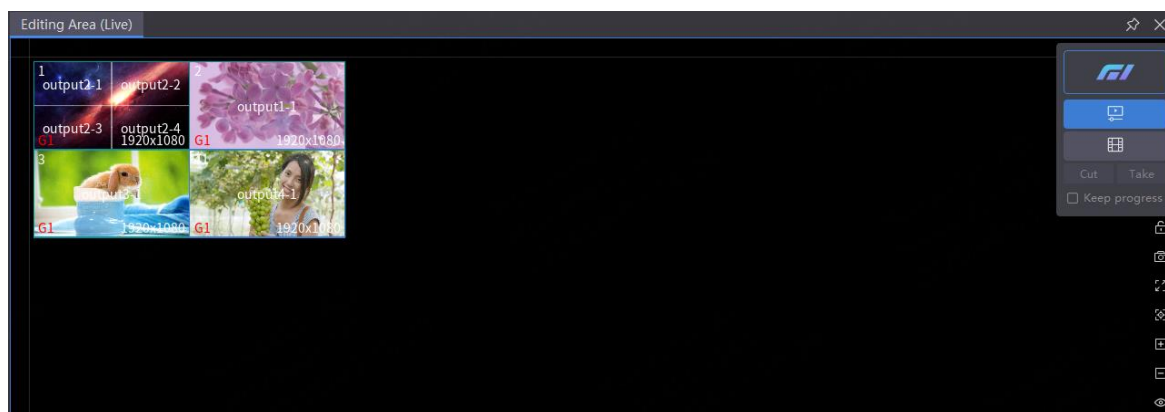
Figure 4-44 Slices
