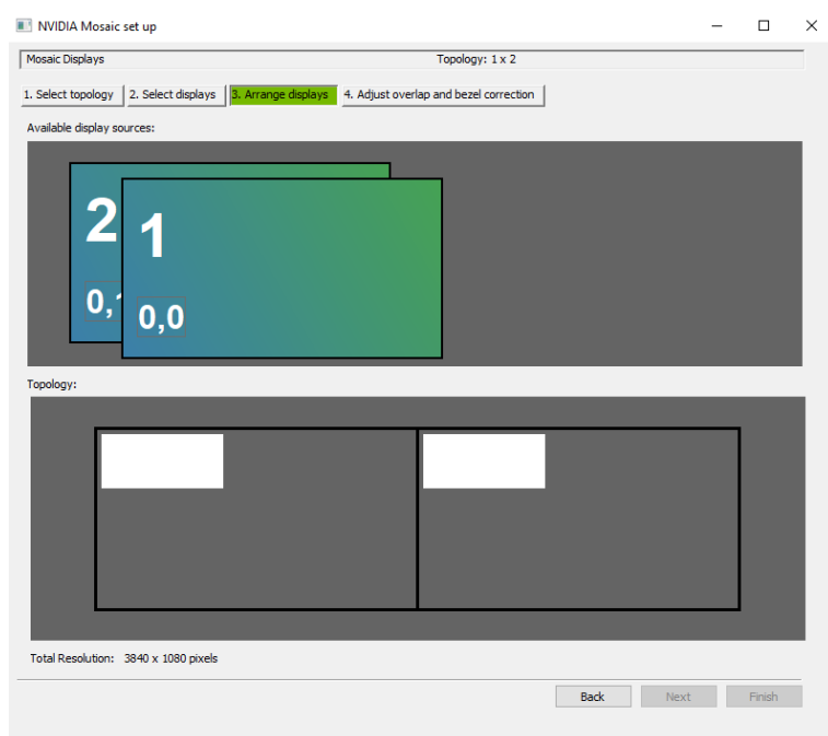
Figure 11-30 Arrange displays
