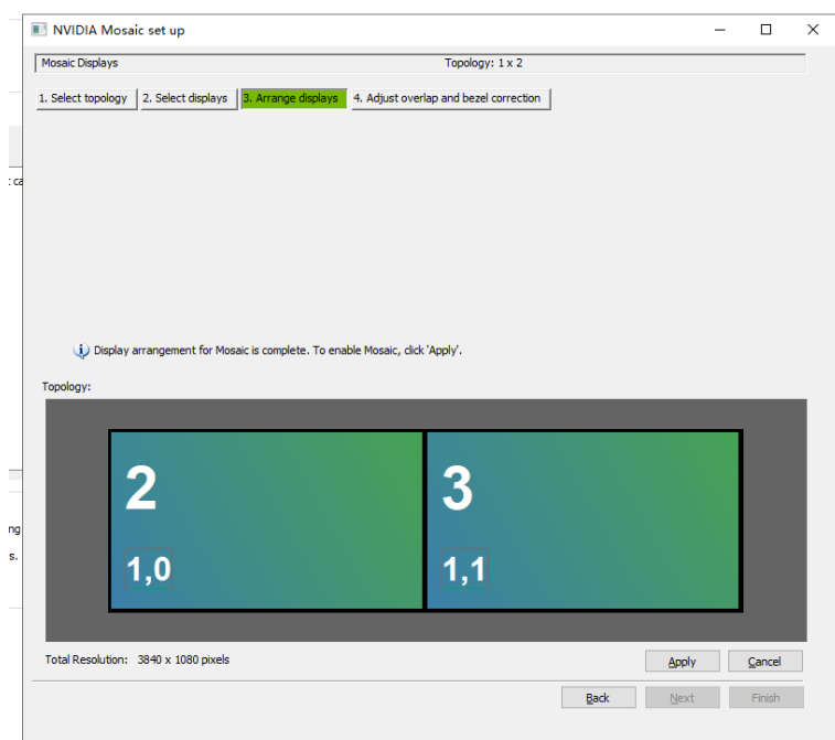
Figure 11-31 Arrange displays
