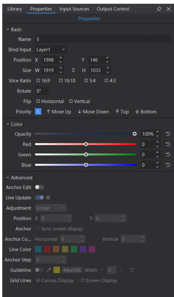
Figure 4-45 Slice properties
