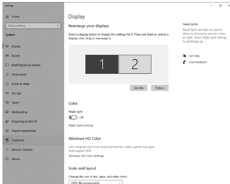
Figure 11-6 Multiple displays-1
