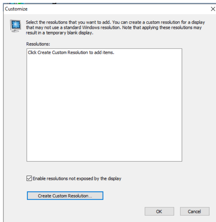
Figure 11-14 Custom resolution-3
