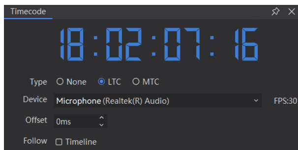
Figure 4-43 Configure timecode
