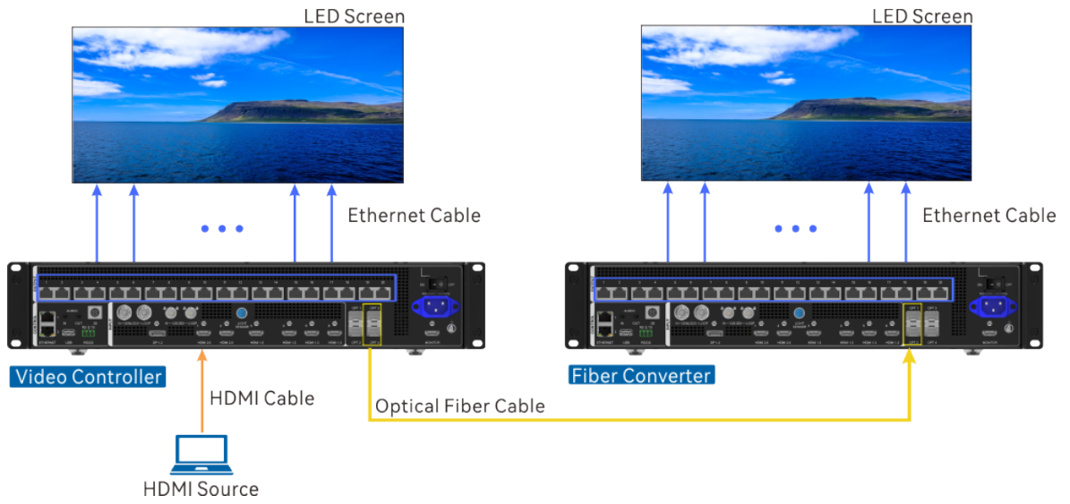
Figure 4-14 Backup between Ethernet and OPT ports
