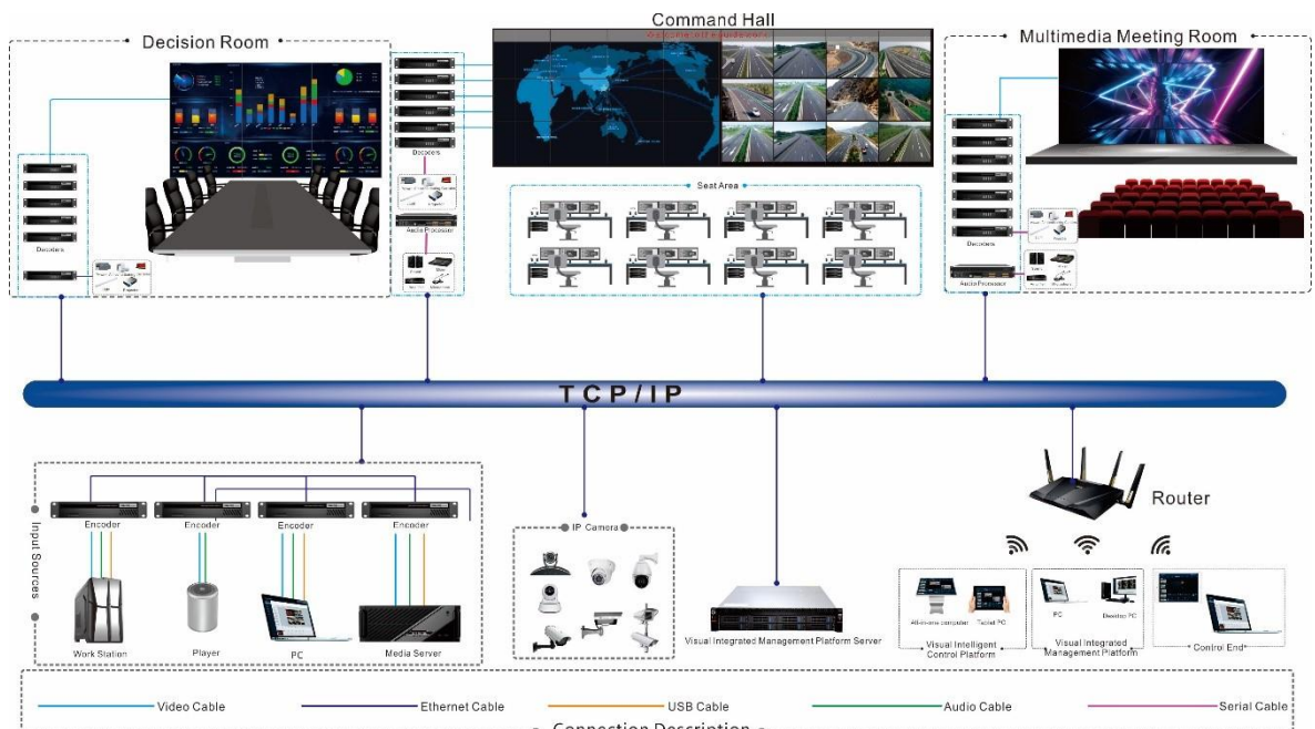
Figure 3-2 Distributed control
