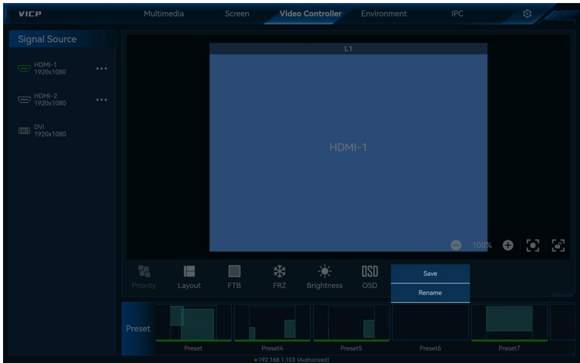
Figure 6-36 Save presets
