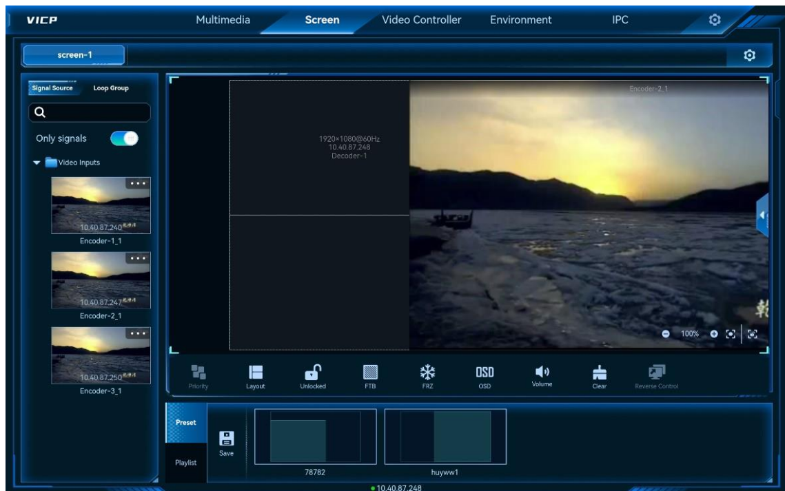
Figure 6-29 Load presets
