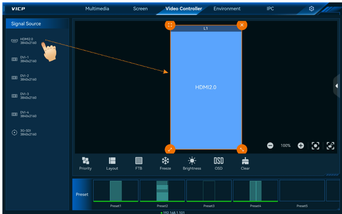
Figure 6-32 Add layers
