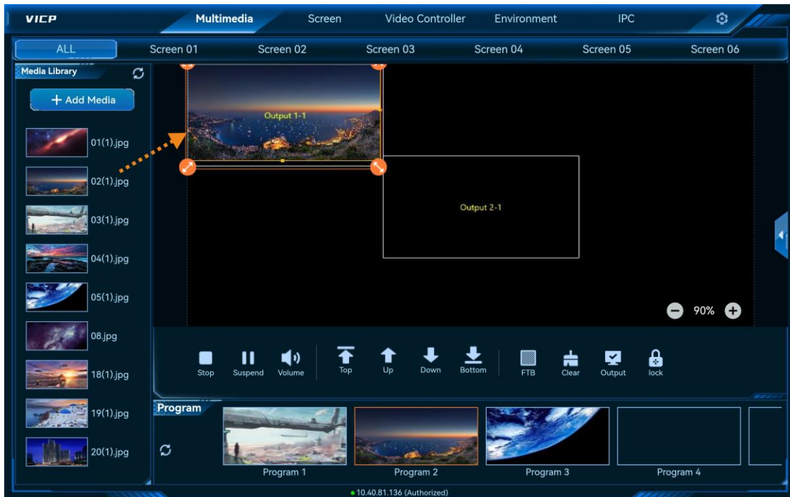
Figure 5-19 Add layers
