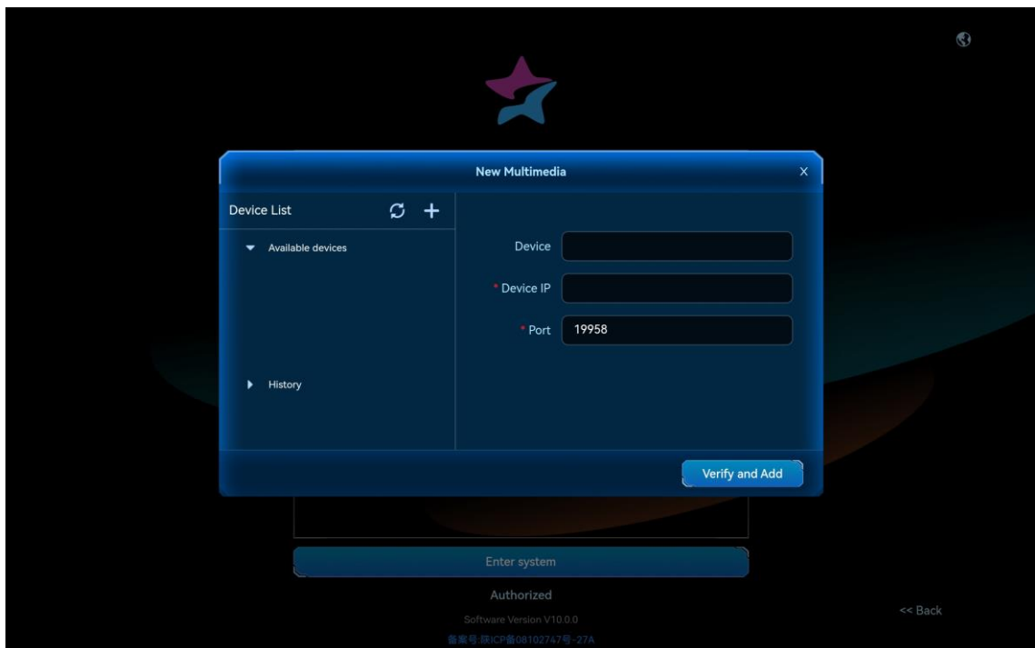
Figure 6-6 New multimedia
