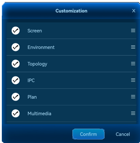
Figure 7-43 Menu customization
