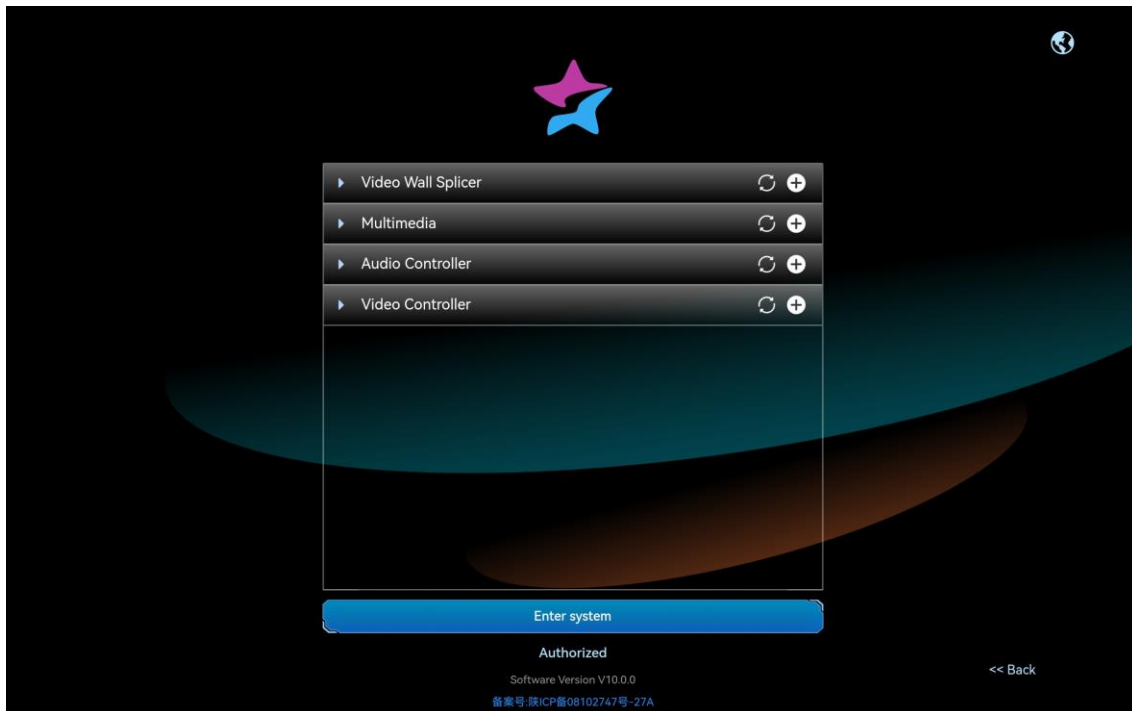
Figure 5-9 Login interface
