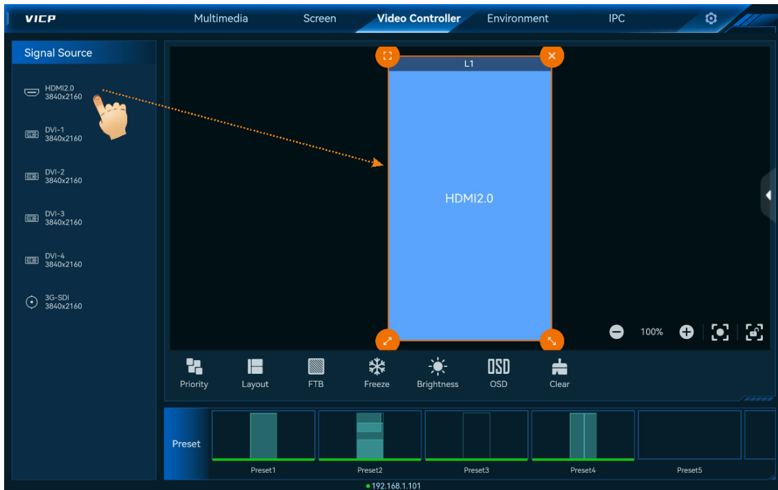
Figure 5-36 Add layers
