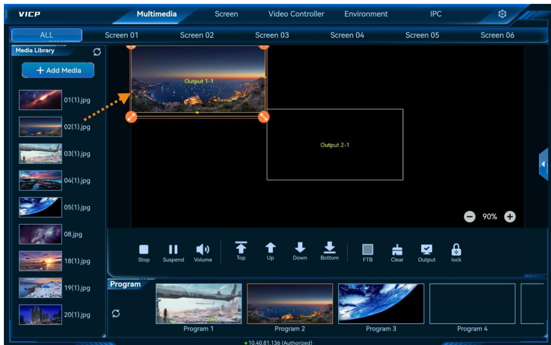
Figure 6-18 Add layers
