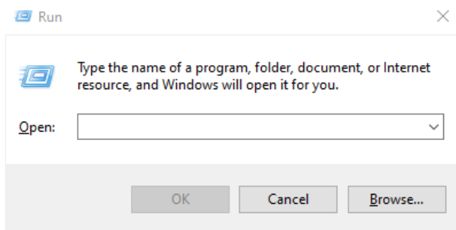
Figure 9-1 Run window
