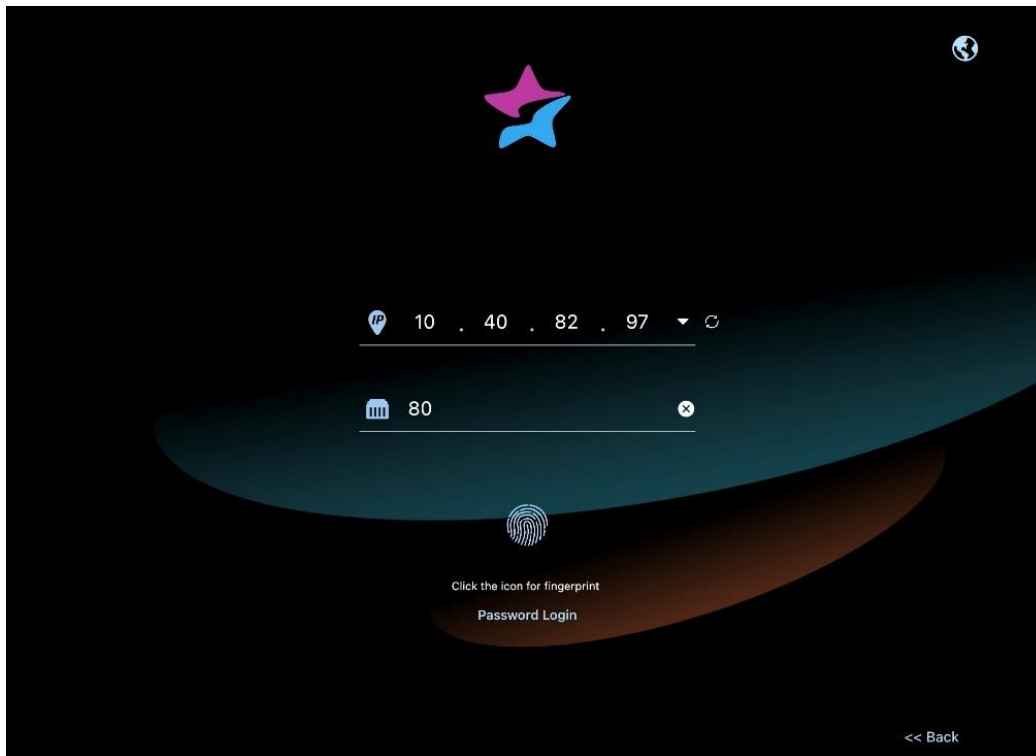
Figure 7-6 Fingerprint login
