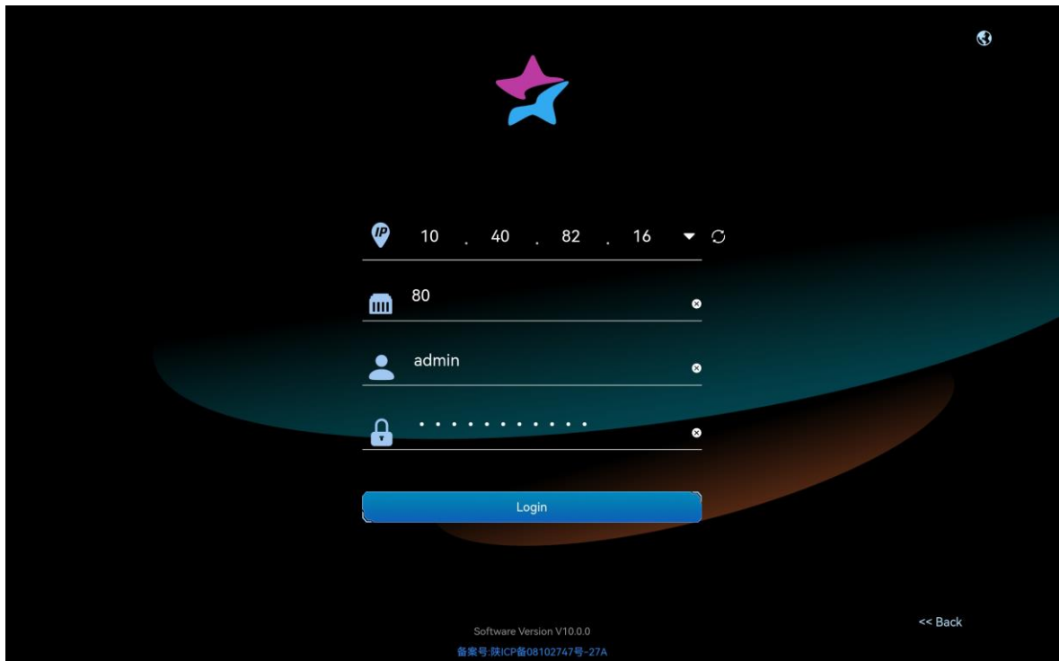
Figure 7-1 Login interface
