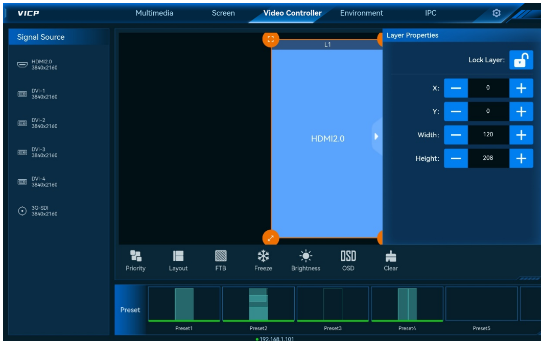
Figure 5-37 Layer properties
