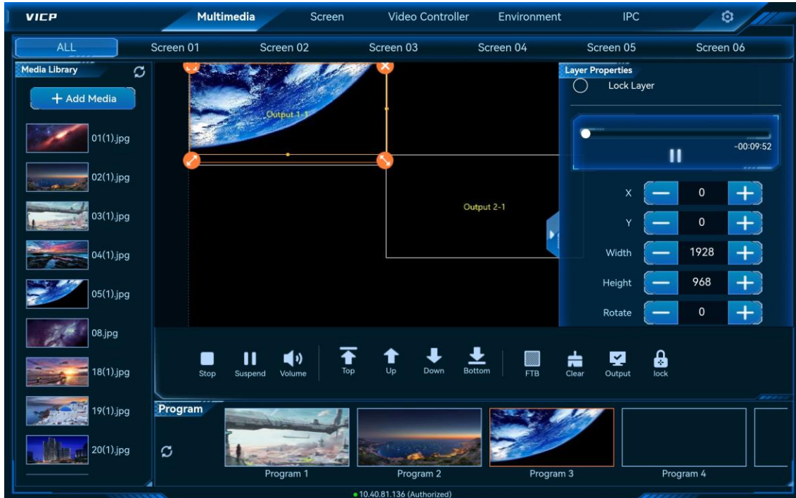
Figure 5-20 Layer properties
