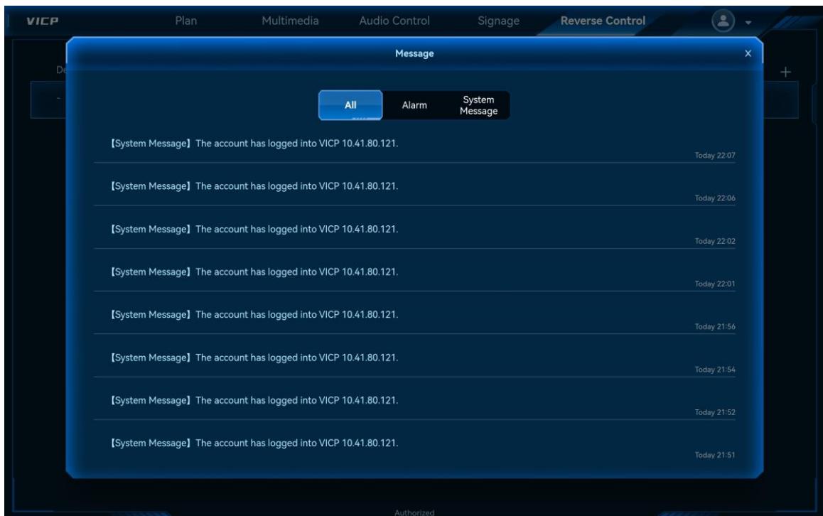
Figure 7-42 Messages
