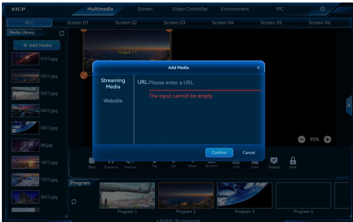
Figure 5-17 Add media
