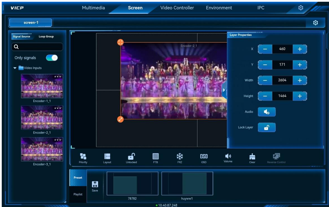
Figure 5-23 Layer properties
