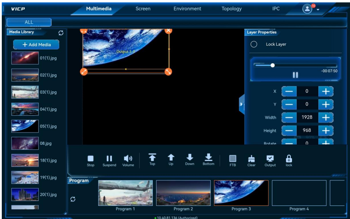
Figure 7-10 Layer properties
