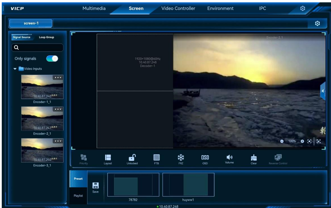
Figure 5-32 Load presets
