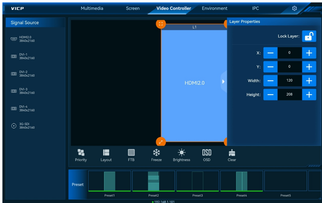
Figure 6-33 Layer properties
