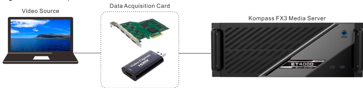
Figure 5-16 Data acquisition card connection
