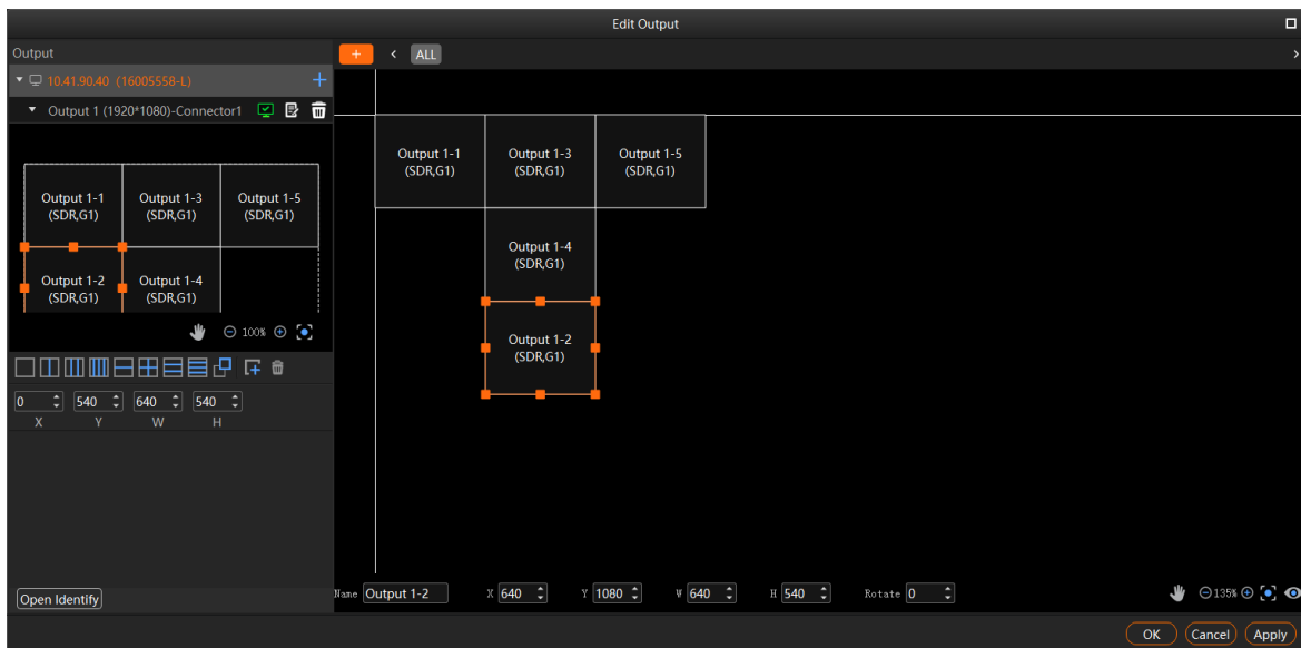
Figure 5-6 Sub-outputs reorganizing
