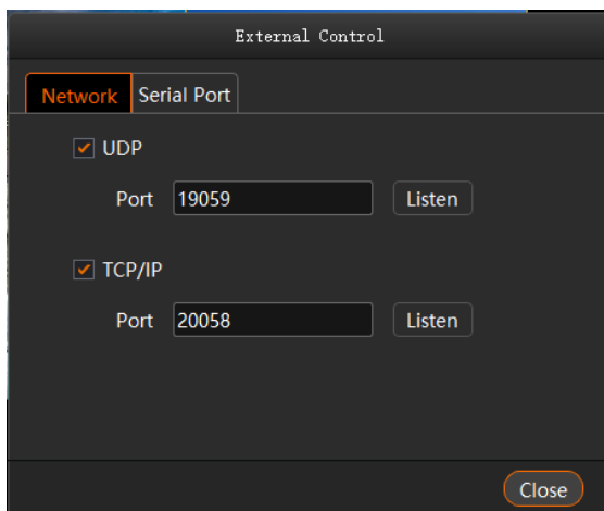
Figure 7-8 Port settings
