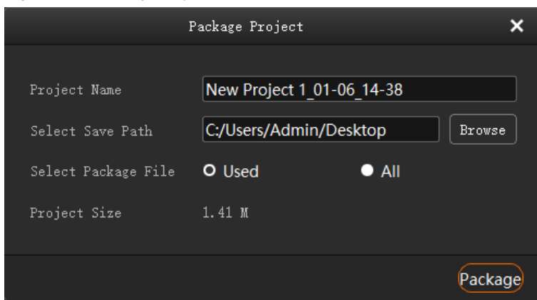
Figure 5-48 Package projects
