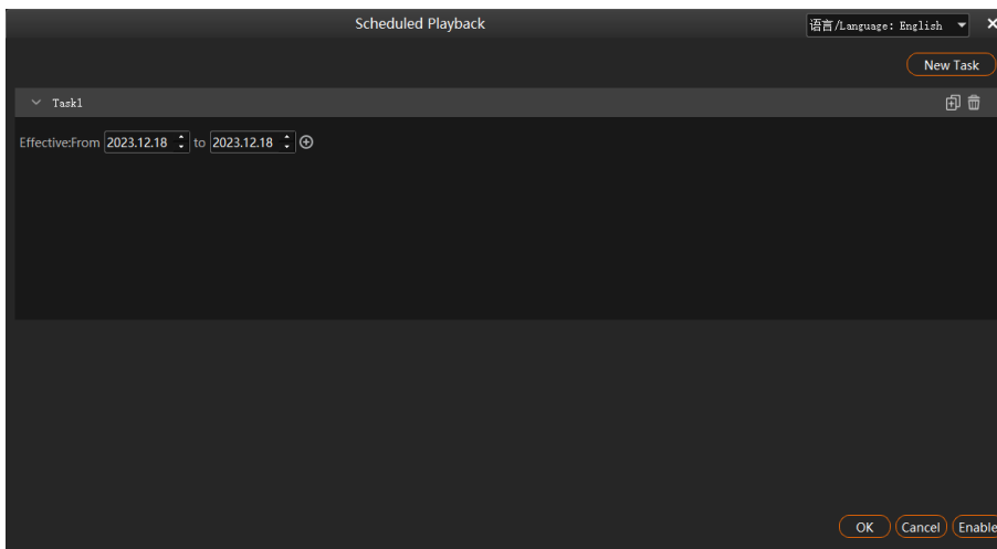
Figure 5-42 Playback tasks
