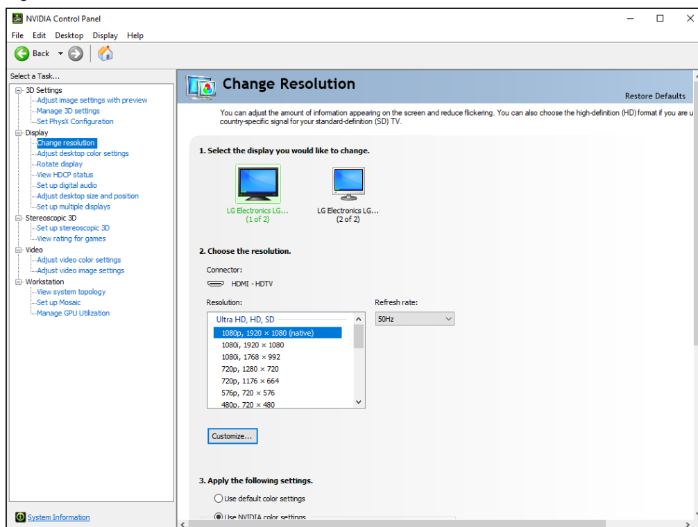
Figure 10-15 Custom resolution-4
