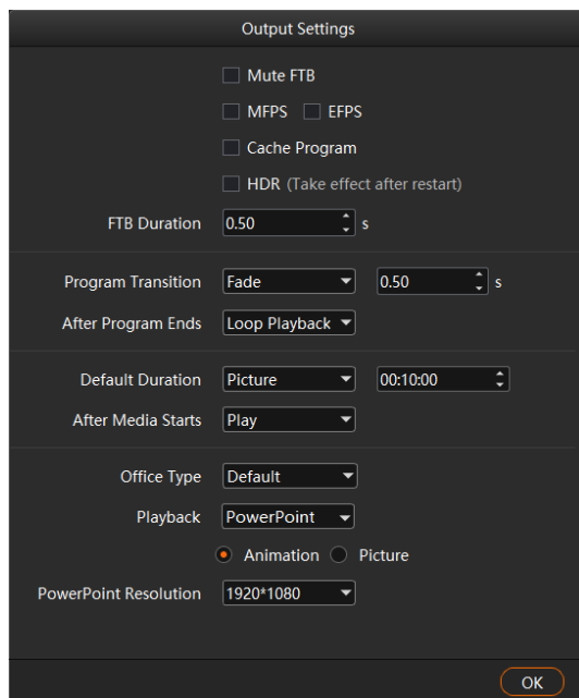
Figure 7-2 Output settings
