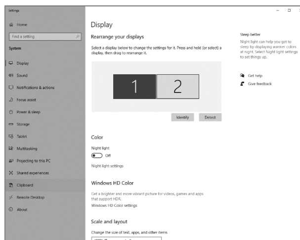
Figure 10-2 Multiple displays-1
