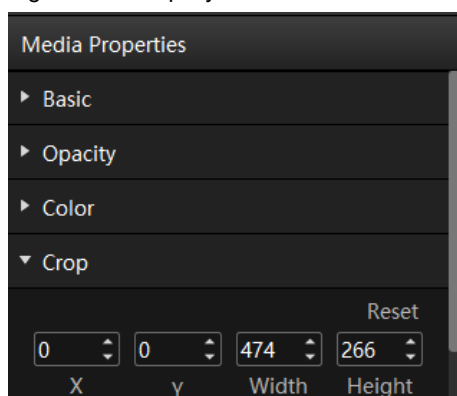
Figure 5-36 Crop layers
