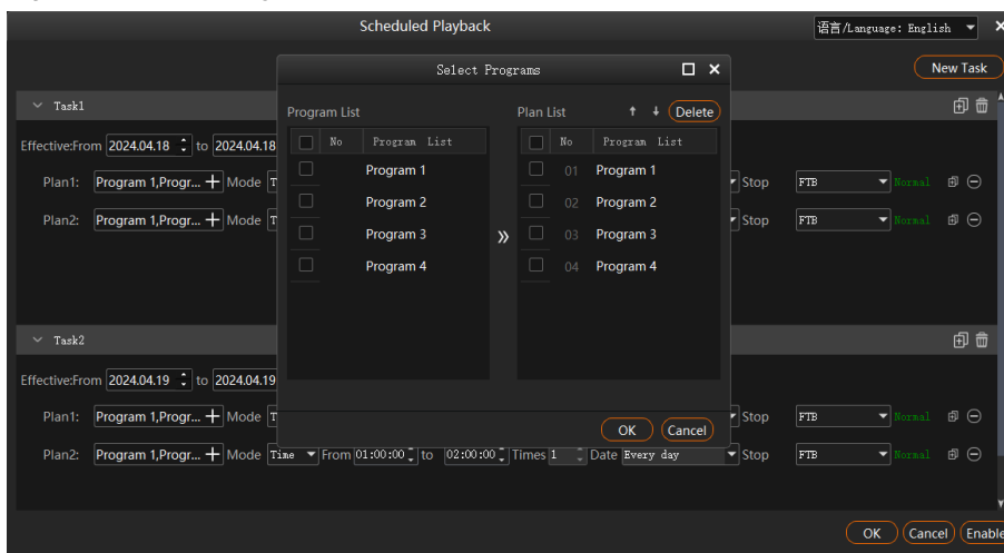
Figure 5-46 Select programs
