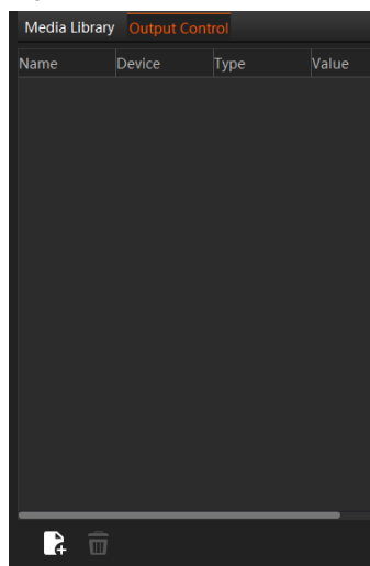
Figure 5-23 Output control
