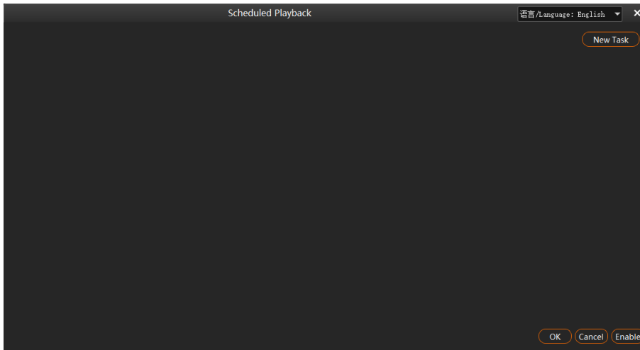
Figure 5-41 Scheduled programs
