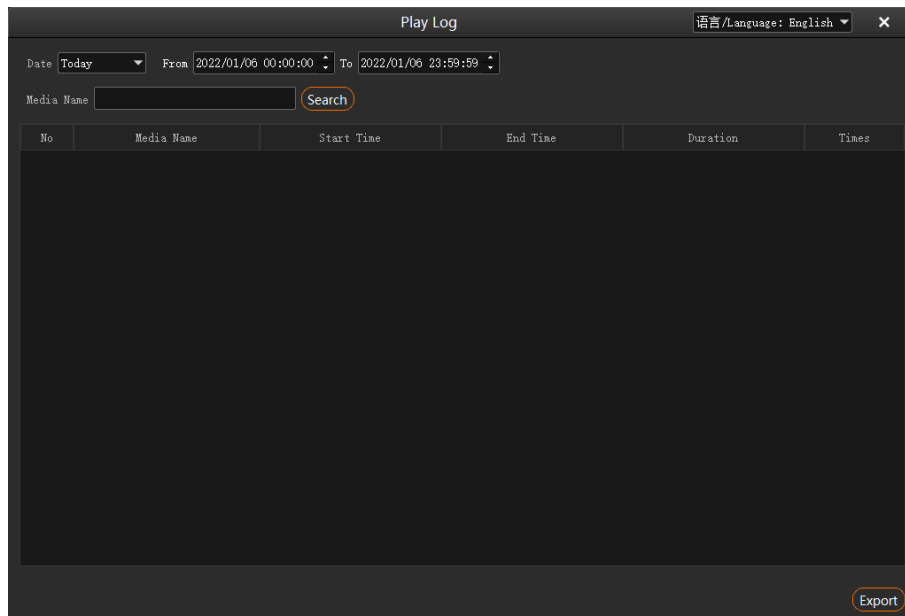
Figure 8-2 Play log
