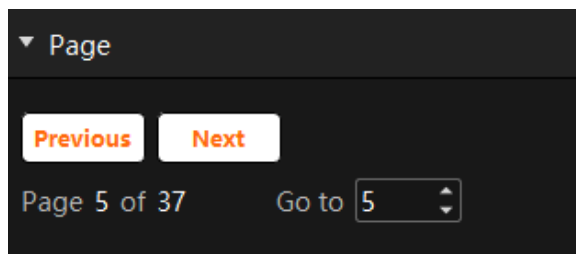
Figure 5-33 Page flipping
