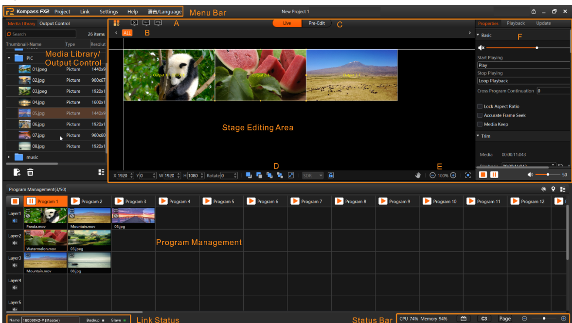
Figure 3-1 User interface
