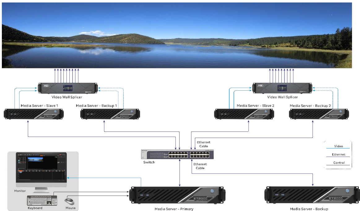
Figure 6-1 Applications
