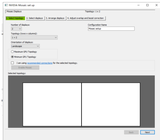
Figure 10-28 Mosaic settings
