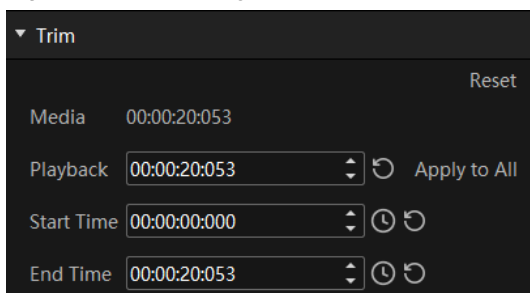
Figure 5-31 Trim settings
