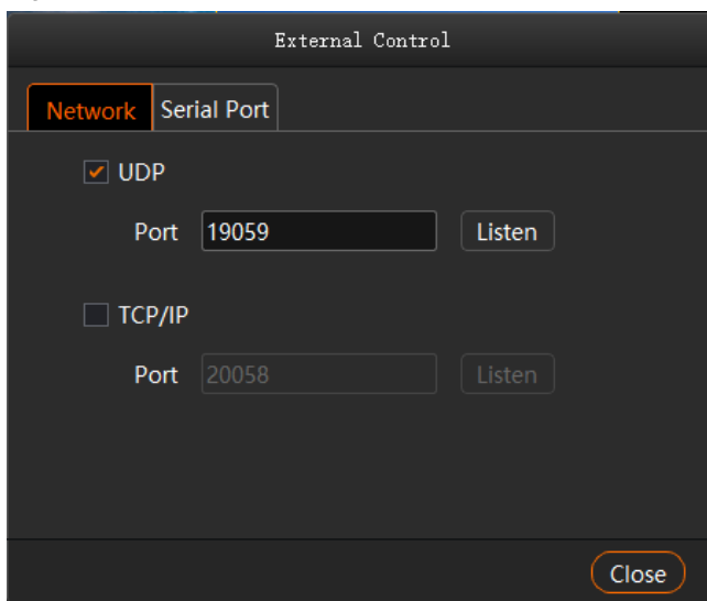
Figure 7-3 External control
