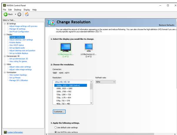
Figure 10-10 Change resolutions
