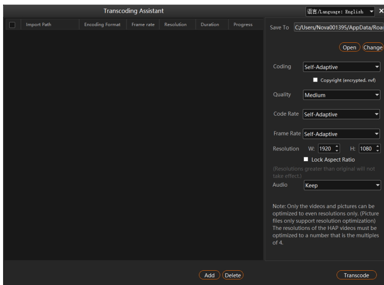
Figure 8-1 Transcoding assistant
