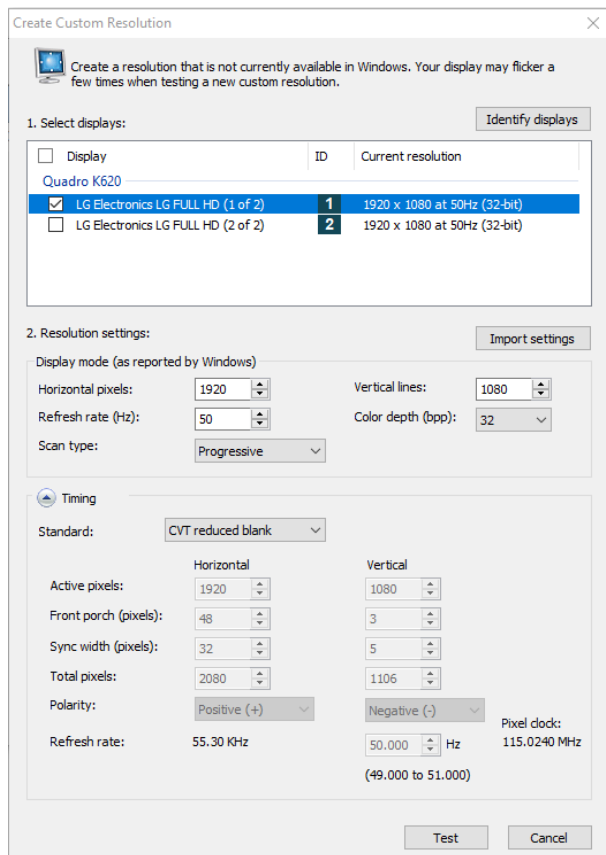
Figure 10-12 Custom resolution-2
