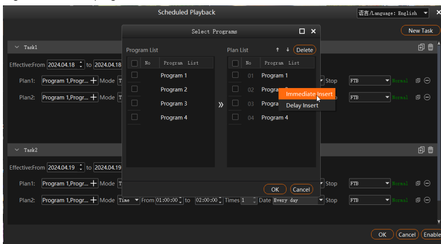
Figure 5-47 Insert programs
