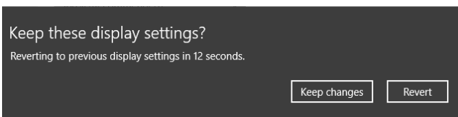
Figure 10-8 Confirmation
