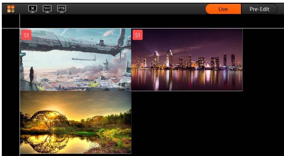
Figure 5-27 Layer group
