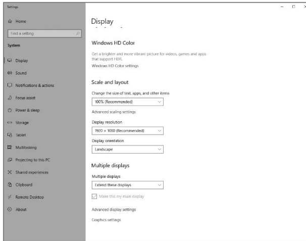
Figure 10-3 Multiple displays-2
