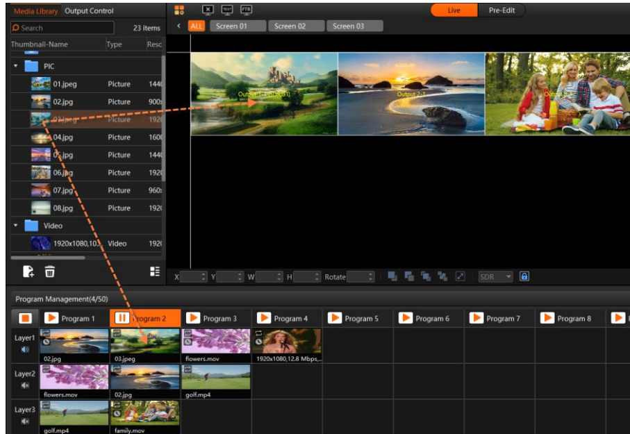
Figure 5-25 Edit programs
