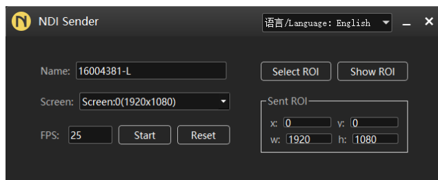
Figure 5-15 NDI Sender
