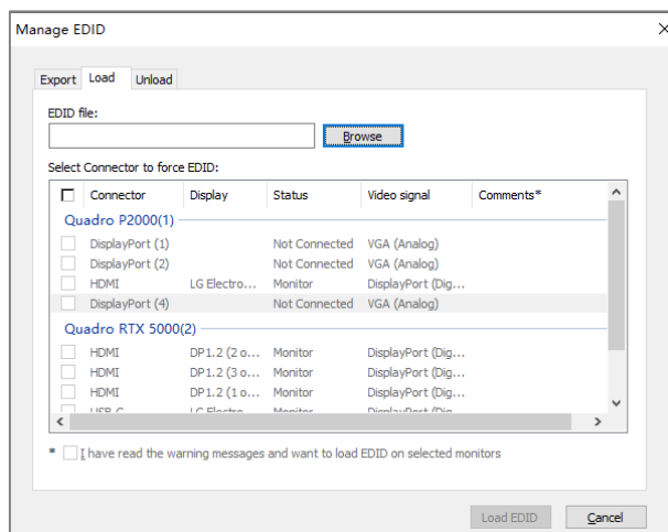
Figure 10-20 Load EDID
