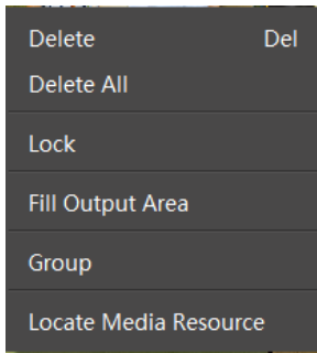
Figure 5-28 Lock media
