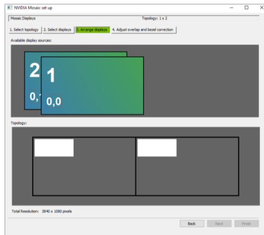
Figure 10-30 Arrange displays
