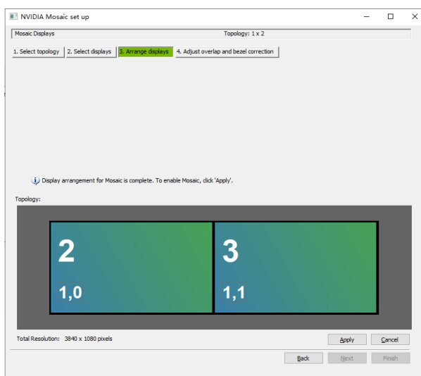
Figure 10-31 Arrange displays
