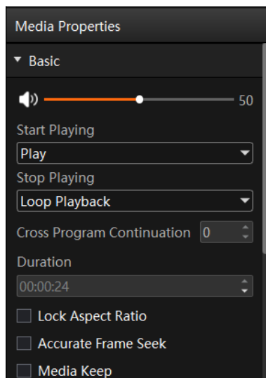
Figure 5-30 Basic properties
