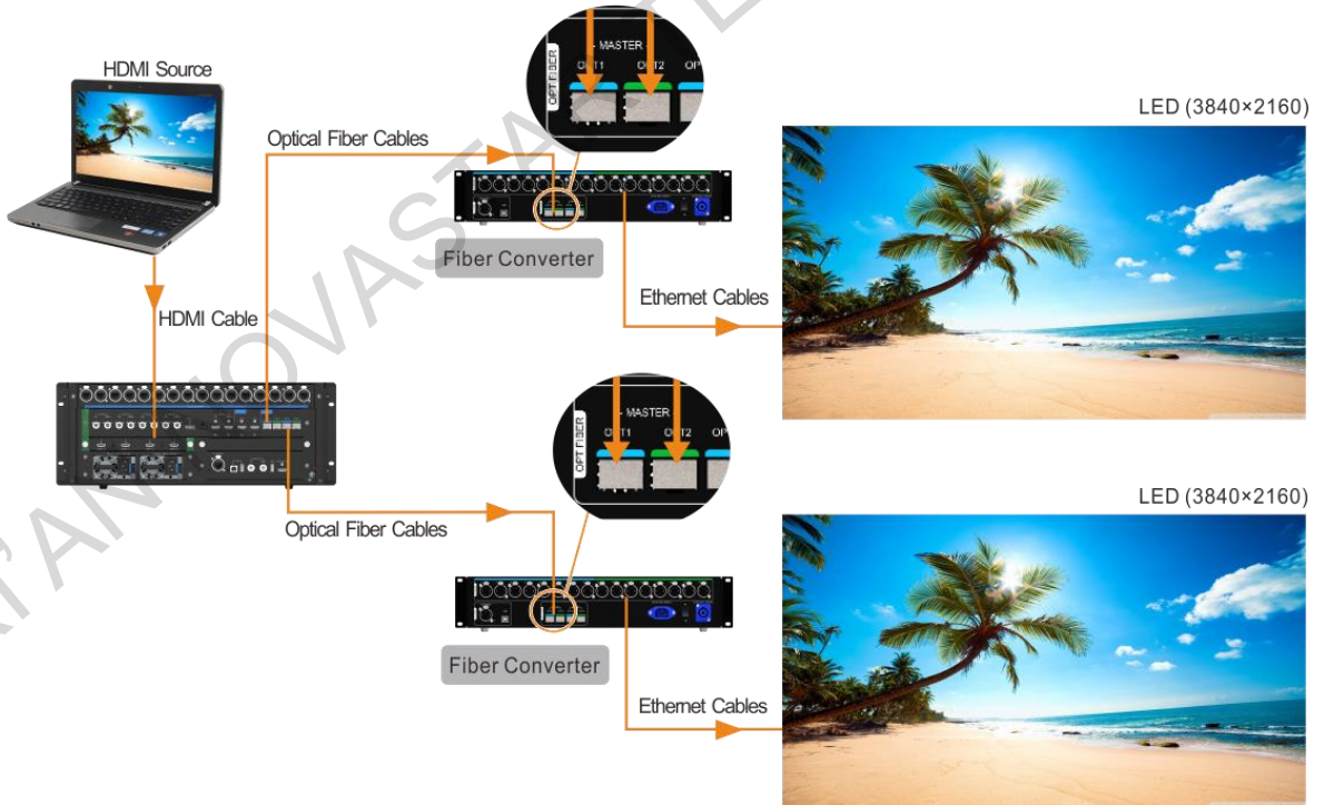
Figure 7-27 Connections for copy mode
