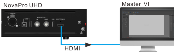
Figure 6-1 Hardware connection
