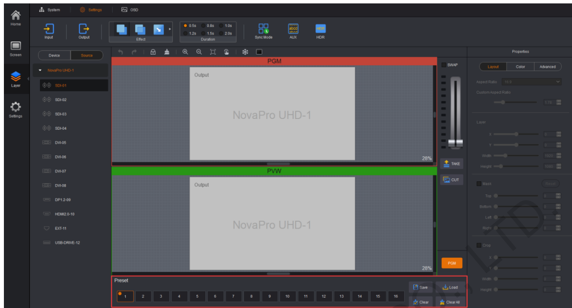
Figure 6-16 Preset settings
