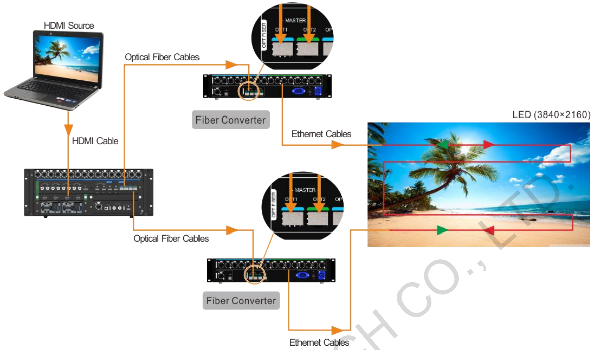
Figure 7-27 Connections for copy mode
