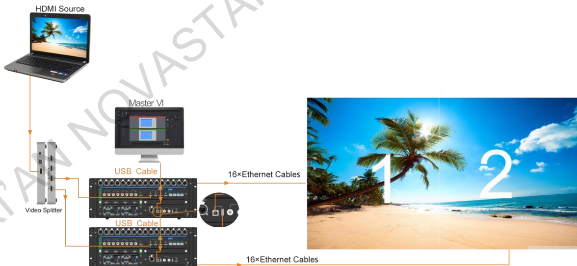
Figure 6-17 Image mosaic
